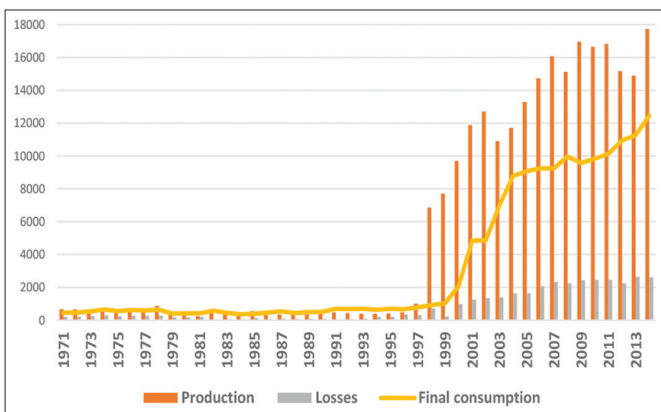
Graph 5: Production, FEC and losses in electricity distribution (GWh)
